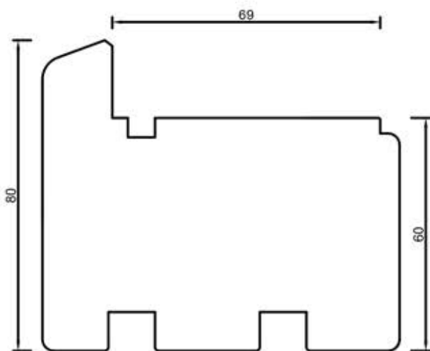
92103 Rama 80 mm
