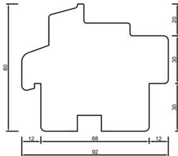
92102 Rama 80 mm
