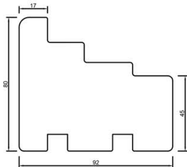
92101 Rama 80 mm
