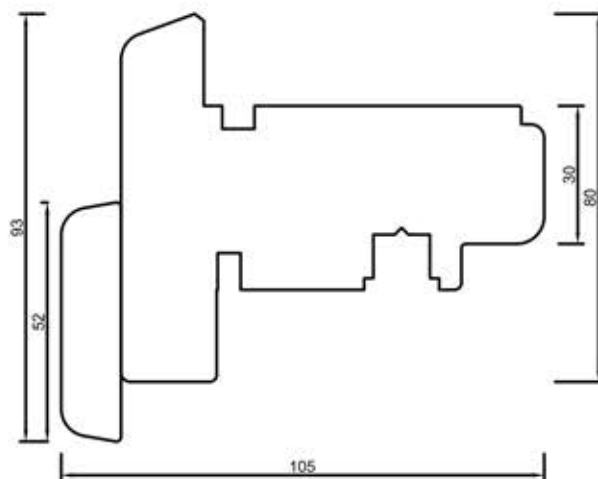
92401 Stulp 52 mm
