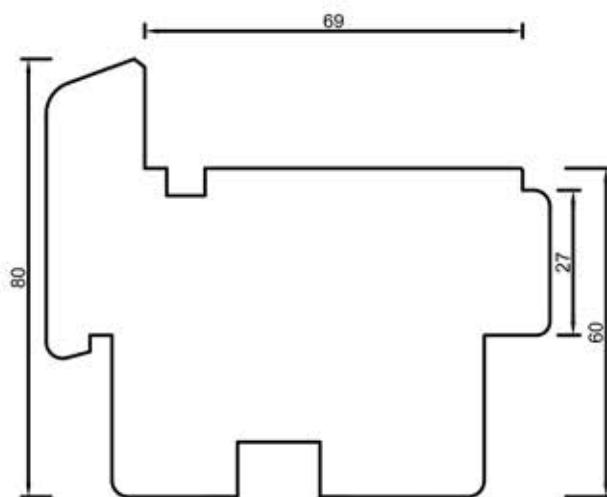
92104 Rama 80 mm
